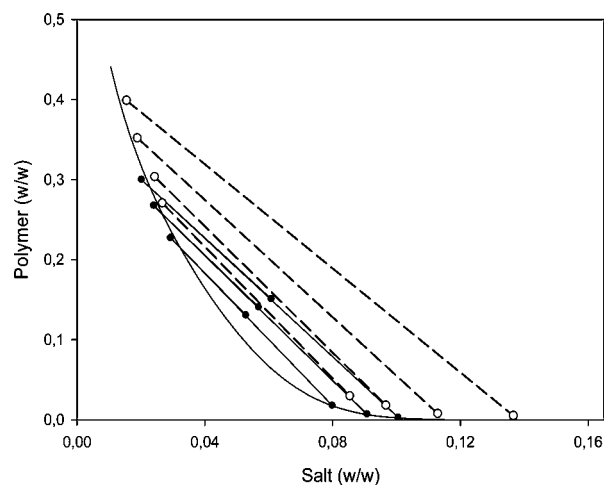
Figure 5. Comparison of the obtained phase diagram for UCON ( M_w = 3900 )–potassium phosphate buffer pH = 7 at 23 °C (▼) with that reported by Li et al. 11 for UCON ( M_w = 4650 )–potassium phosphate buffer pH = 6.8 at 25 °C (○).
